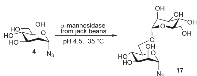
Scheme 3. Transglycosylation reaction with azide donor 4 .
