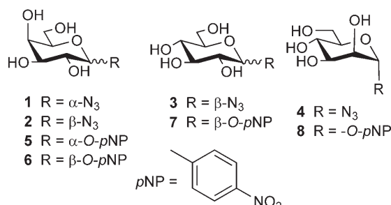
Figure 1. Glycosyl azides 1–4 and respective p -nitrophenyl glycosides 5–8 .
