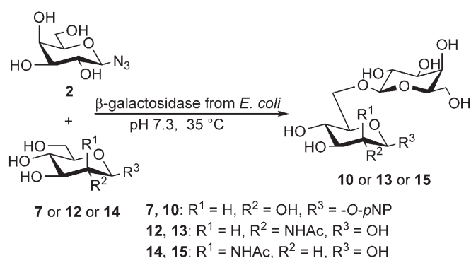
Scheme 1. Transglycosylation reactions with azide donor 2 .
