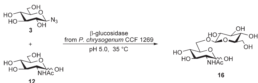
Scheme 2. Transglycosylation reaction with azide donor 3 .
